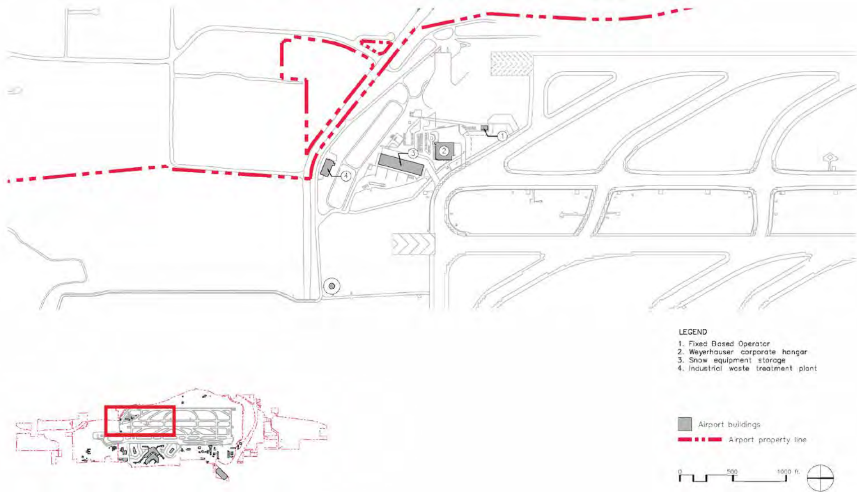
Figure 8-1 General Aviation Facilities Seattle-Tacoma International Airport
